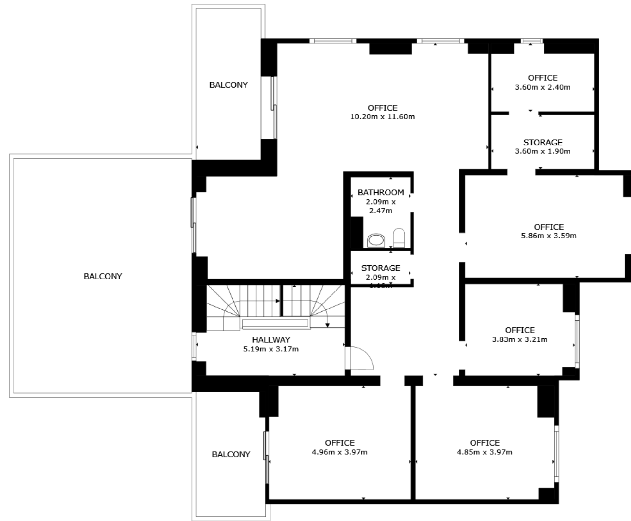
FLOOR 2
